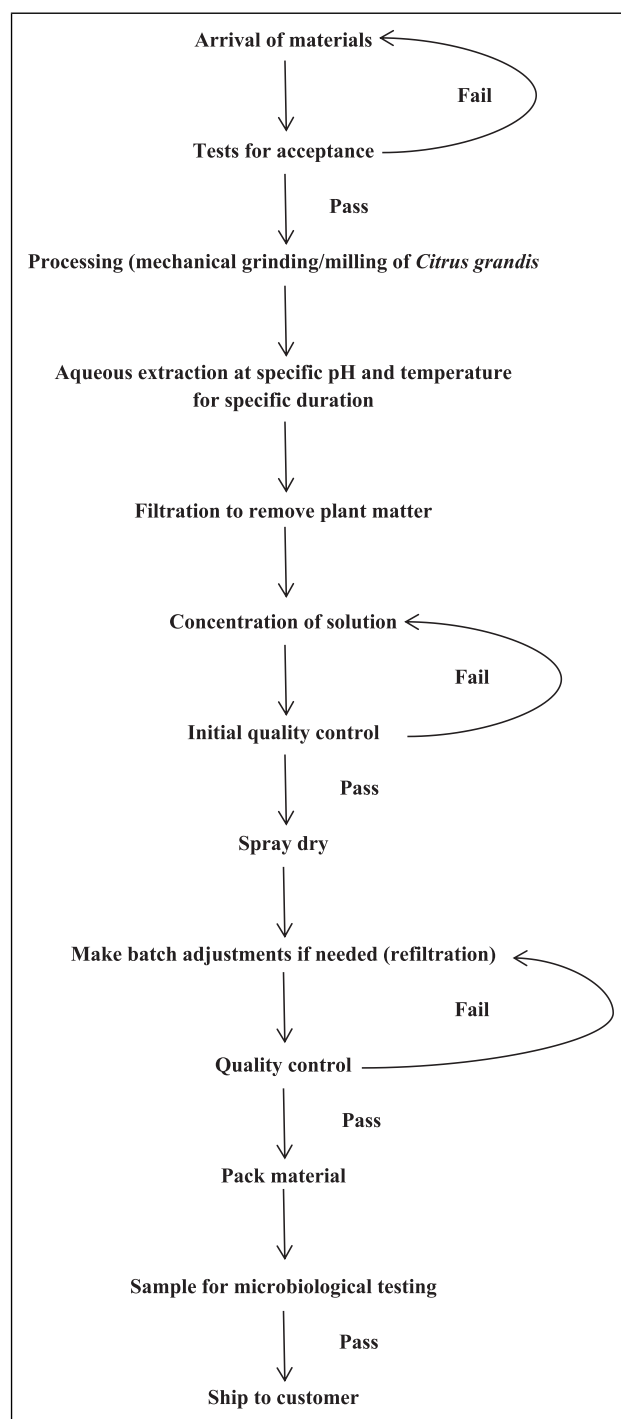
Figure 3. Manufacturing flow chart for Citrus Grandis (Grapefruit) Fruit Extract—Powder Form. 48
