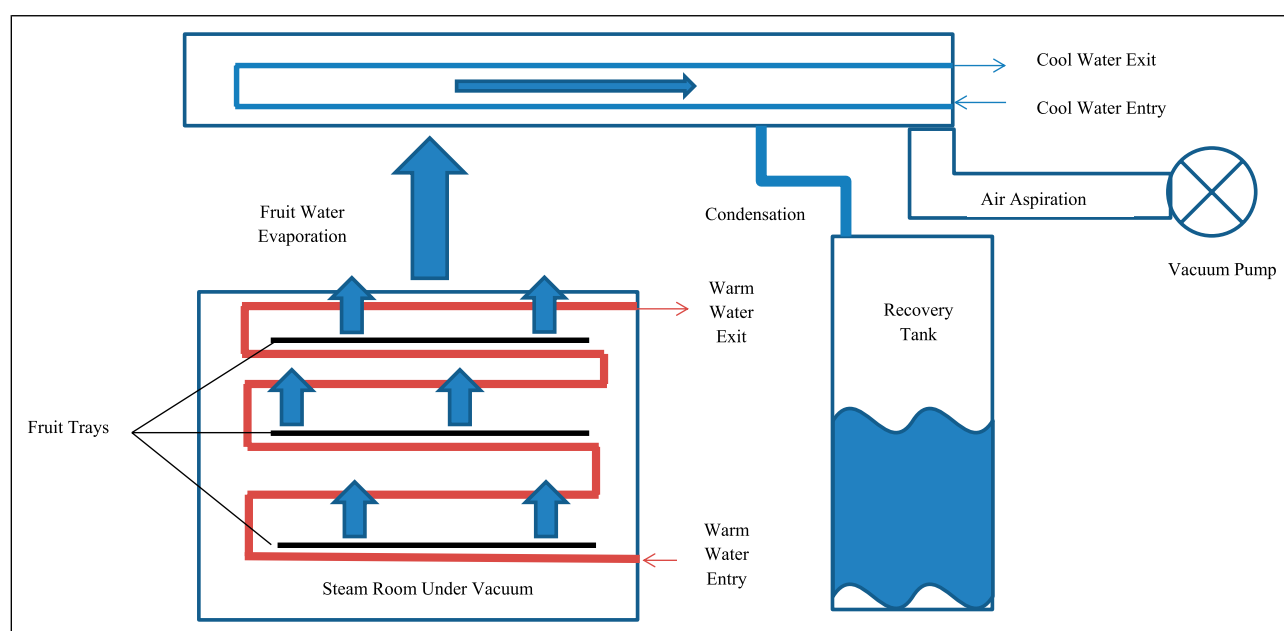
Figure 1. Method of manufacturing of fruit waters. 46
