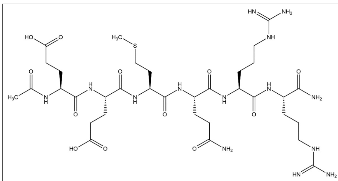
Figure 1. Acetyl Hexapeptide-8 Amide.
