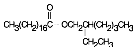
FIGURE 3 Octyl Stearate.
