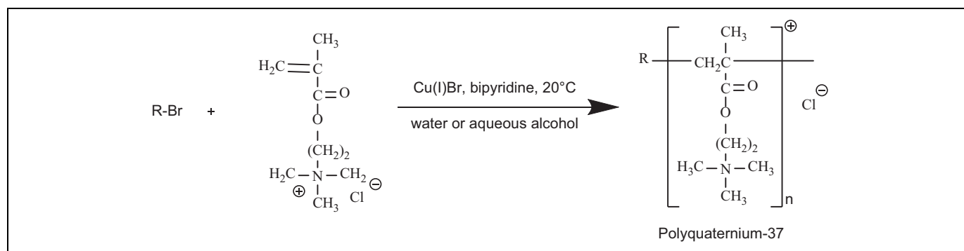
Figure 3. Example synthesis of trimonium decorated polymers (Polyquaternium-37).
