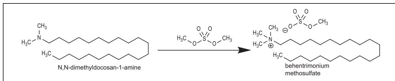
Figure 2. Example synthesis of alkyl trimoniums (behentrimonium methosulfate).
