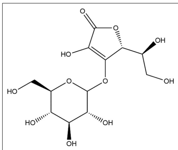
Figure 1. Ascorbyl Glucoside.
