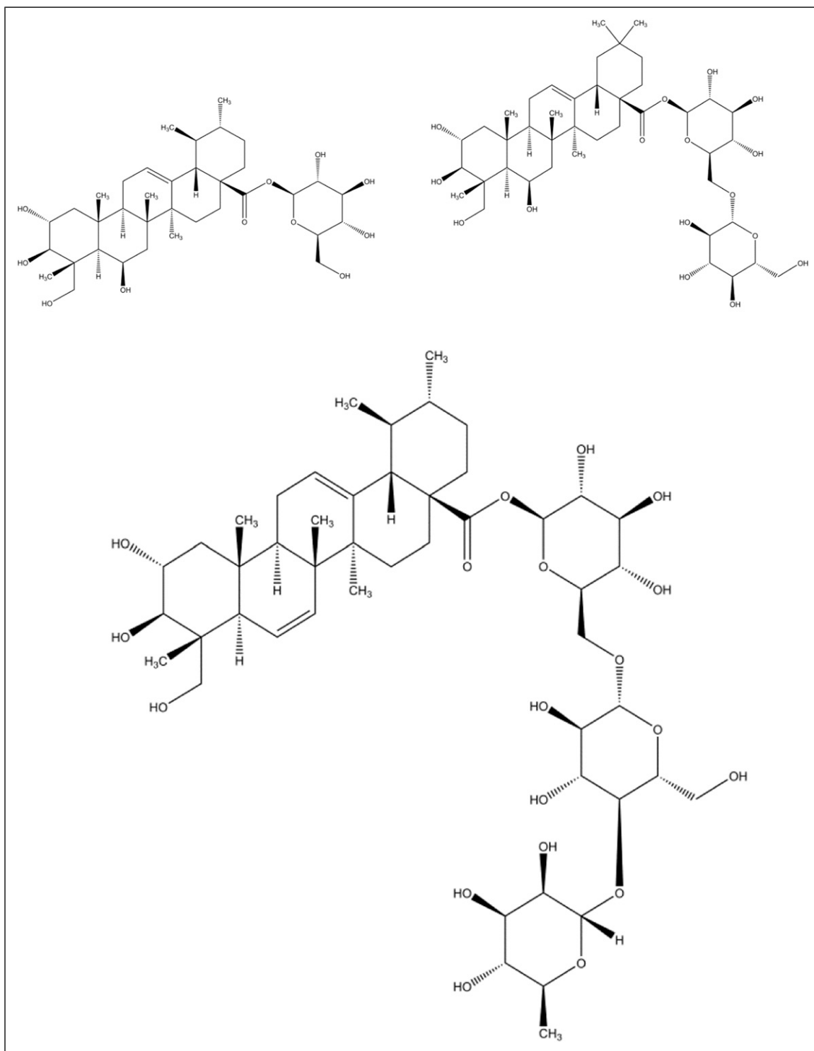
Figure 3. Centellosides.
